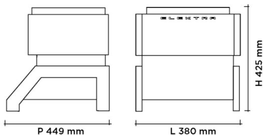
VERVE 1 Group Semi-automatic Stainless Steel/Wood
